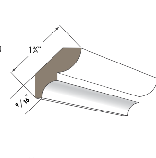
Bed Moulding AZM-75 Length: 16'
