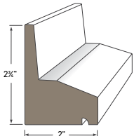
Water Table AZM-6935 Length: 18'
