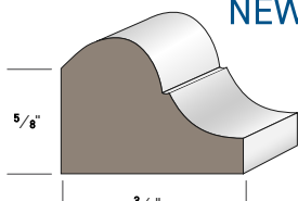
Nose Cove AZM-7480 Length: 16'
